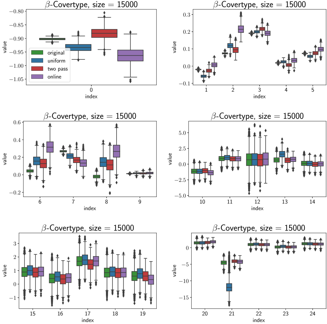
Figure 8: The posterior samples obtained after running each of the algorithms for a reduction size of 15000 are compared to the original sample of the posterior distribution of the Covertypes dataset by using boxplots for each of the dimensions of \beta . Here, we can see \beta_0 to \beta_{24} , the remainder can be found in Figure 9.
