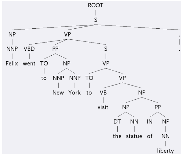
Figure 1.6: The constituent parse tree of the sentence "Felix went to New York to visit the statue of liberty."
