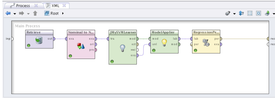
Figure 1.2: Exemplary process in RapidMiner
