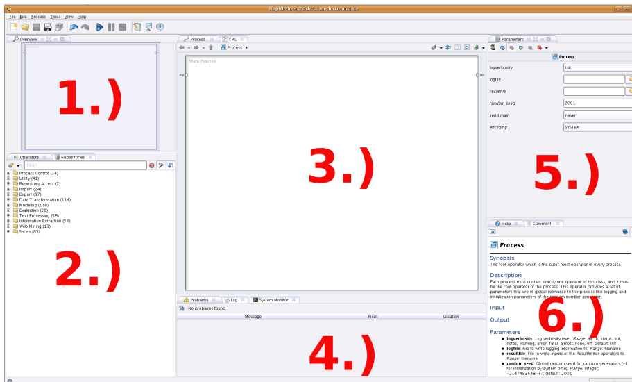
Figure 1.1: RapidMiner graphical user interface
