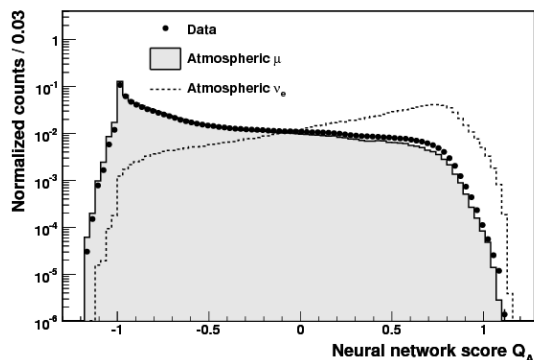
FIG. 6: Normalized distributions of the Level-4 neural network classification score.
