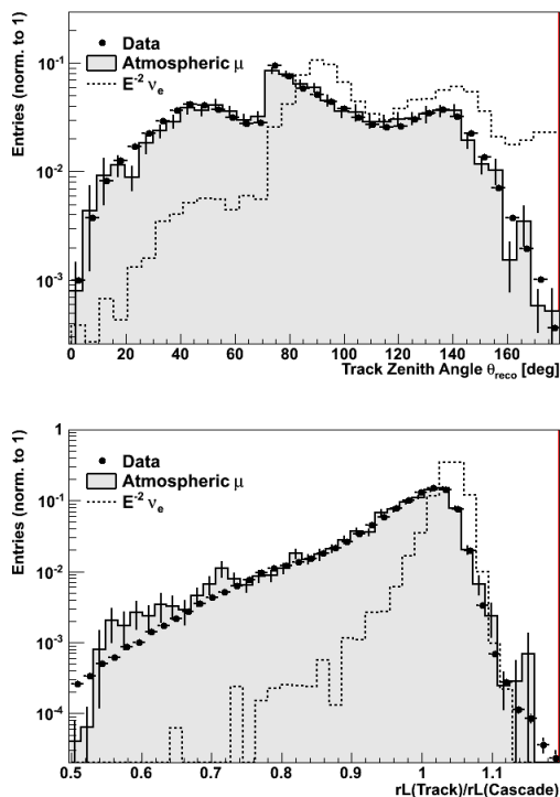
FIG. 2: Normalized distributions of (top) zenith angle and (bottom) reduced log likelihood ratios after Level-5 event selections for the data (filled circles), muon background Monte Carlo (continuous histogram) and signal neutrino (dashed histogram).
