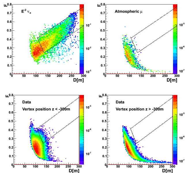
FIG. 5: (Color online) The fill-ratio, F , versus the distance, D , as defined in the text for (top-left panel) the Monte Carlo simulated signal sample, (top-right panel) the Monte Carlo simulated muon background sample, and the data at the bottom part of the detector (bottom-left panel) and at the top part of the detector (bottom-right panel). The right axis shows the rate [Hz]. The dashed lines show the selection boundaries applied at Level-7 in the analysis.
