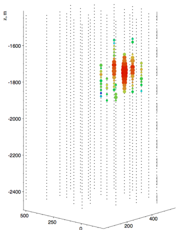
FIG. 15: (Color online) The MC muon background event which passed all selections in extraterrestrial analyses and which has the reconstructed energy of 18 TeV is displayed from the side. Different colors of the circles represent different DOMs hit times, with early hits in red and late hits in blue. The size of the circles represents the amplitude.
