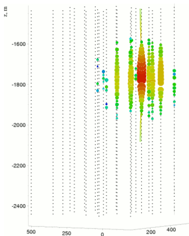
FIG. 16: (Color online) The data event which passed all selections in atmospheric and extraterrestrial analyses and which has the highest reconstructed energy of 134 TeV is displayed from the side. Different colors of the circles represent different DOMs hit times, with early hits in red and late hits in blue. The size of the circles represents the amplitude.
