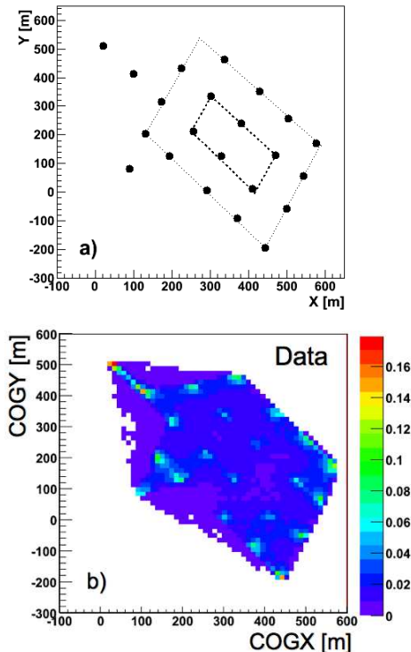
FIG. 1: (Color online) a) The filled circles show the positions of the strings in the x - y (horizontal) plane for the 22-string detector configuration. The lines show the boundaries of the fiducial volume and are described in the text. b) The reconstructed center-of-gravity position x (COGX) versus y (COGY) for events passing the cascade online filter. The right axis shows the rate [Hz].
