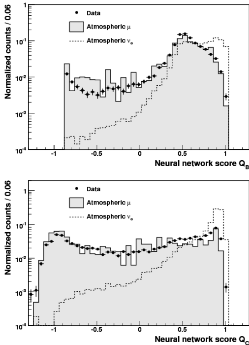
FIG. 9: Normalized distributions of the neural network classification scores (top) Q_B and (bottom) Q_C .
