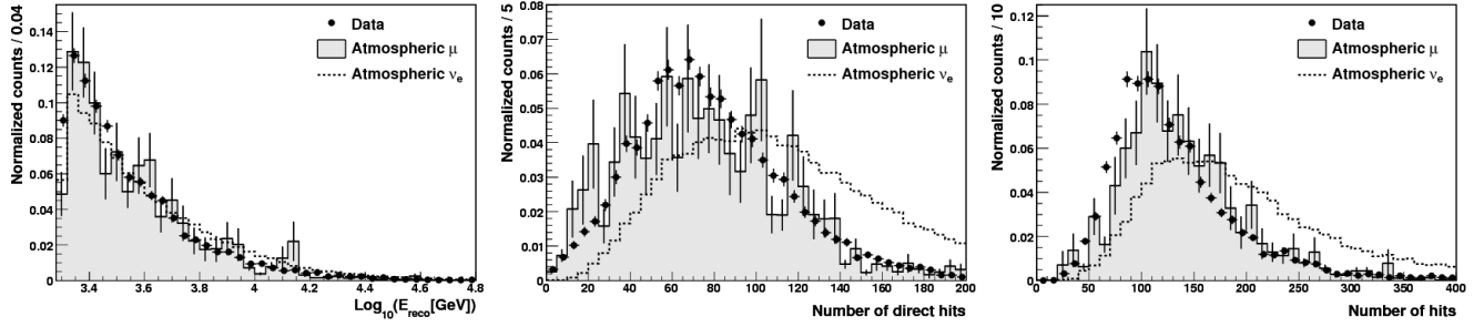
FIG. 7: Normalized distributions (after Level-4 atmospheric selections) of (left panel) reconstructed energy (middle panel) number of direct hits (right panel) total number of hits.
