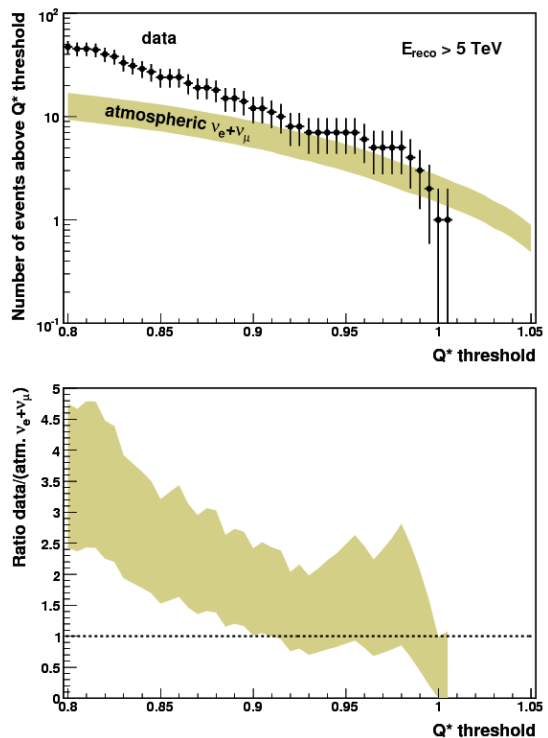
FIG. 12: Experimental events reconstructed with energies above 5 TeV in the atmospheric analysis compared to an expected cascade signal from atmospheric neutrinos. (top) The cumulative number of events above a threshold in the multivariate selection parameter Q^* for data and simulated signal. (bottom) The ratio of data to expected signal as a function of selection threshold.
