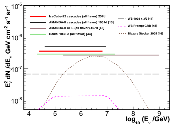
FIG. 14: (Color online) Experimental upper limits on the diffuse flux of neutrinos from sources with \Phi \propto E^{-2} energy spectrum and theoretical predictions for neutrino fluxes from astrophysical neutrino sources.
