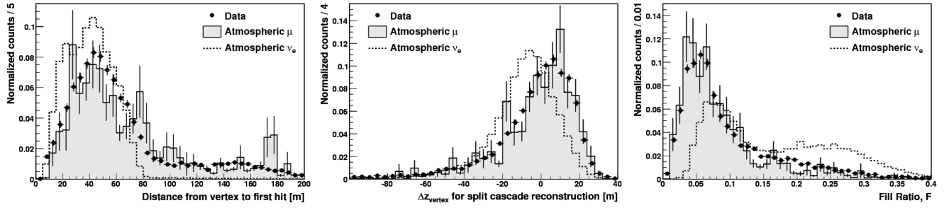
FIG. 8: Normalized distributions (after Level-4 atmospheric selections) of (left panel) distance from the cascade vertex to the first hit in the event (middle panel) difference in z vertex positions for the two split cascade reconstructions (right panel) fill-ratio from the mean hit distance.
