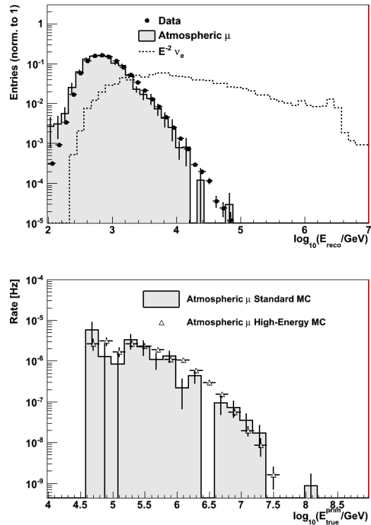
FIG. 3: (top) Normalized distribution of the reconstructed cascade energy after level-6 event selections for the data (filled circles), muon background Monte Carlo (continuous histogram) and signal neutrino (dashed histogram). (bottom) Absolute event rate versus primary Cosmic Ray energy after level-6 event selections with an additional selection criterion on the reconstructed cascade energy of 6.3 TeV for the standard Corsika Monte Carlo (continuous histogram) and high-energy optimized Corsika Monte Carlo (open triangles).
