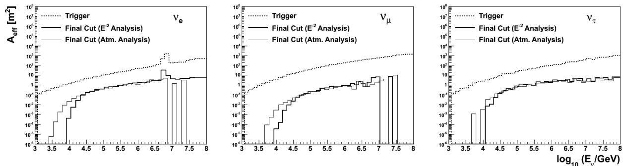
FIG. 10: The effective area, A_{\text{eff}} , for (left panel) \nu_e , (middle panel) \nu_\mu , and (right panel) \nu_\tau versus neutrino energy at trigger level (dashed curves) and at analysis level after all selections for both the extraterrestrial and the atmospheric analysis (continuous curves).
