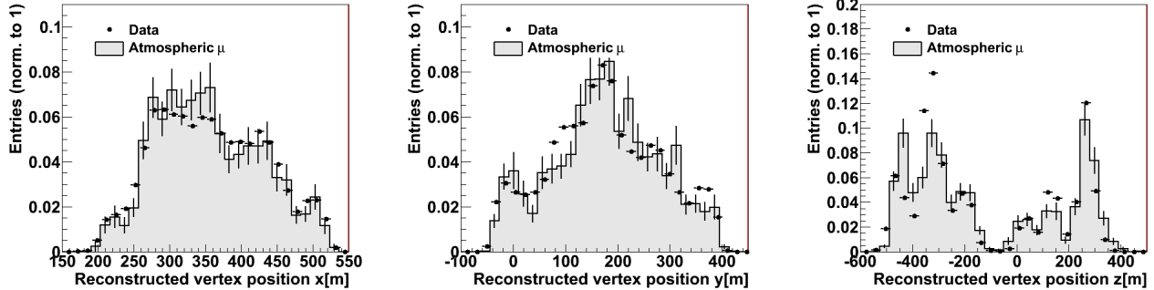
FIG. 4: Normalized distributions of cascade reconstructed vertex position: x component (left panel), y component (middle panel) and z component (right panel) after level-6 event selections for the data (filled circles), standard muon background Monte Carlo (continuous histogram).
