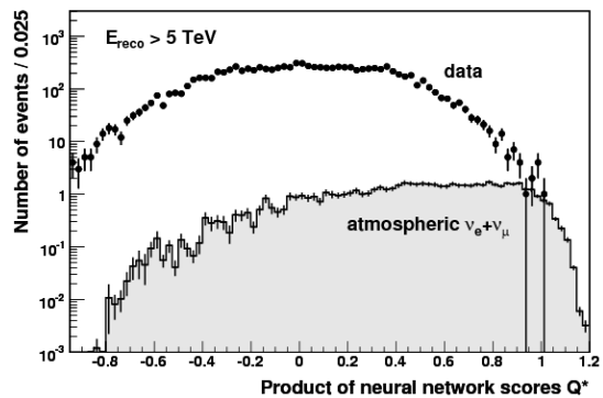
FIG. 11: Distribution of the multivariate selection parameter Q^* for data and for a simulated cascade signal from \nu_e and \nu_\mu with reconstructed energies above 5 TeV in the atmospheric analysis.
