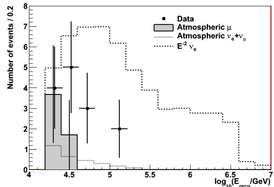
FIG. 13: Cascade reconstructed energy distribution after all selections in the extraterrestrial analysis.
